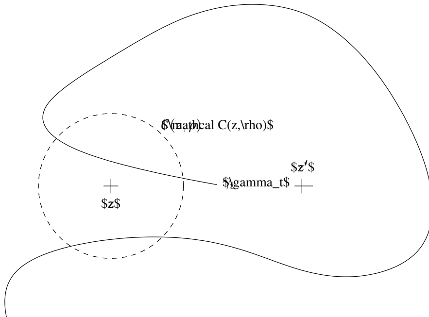
Figure 2: Proof of Lemma 6
